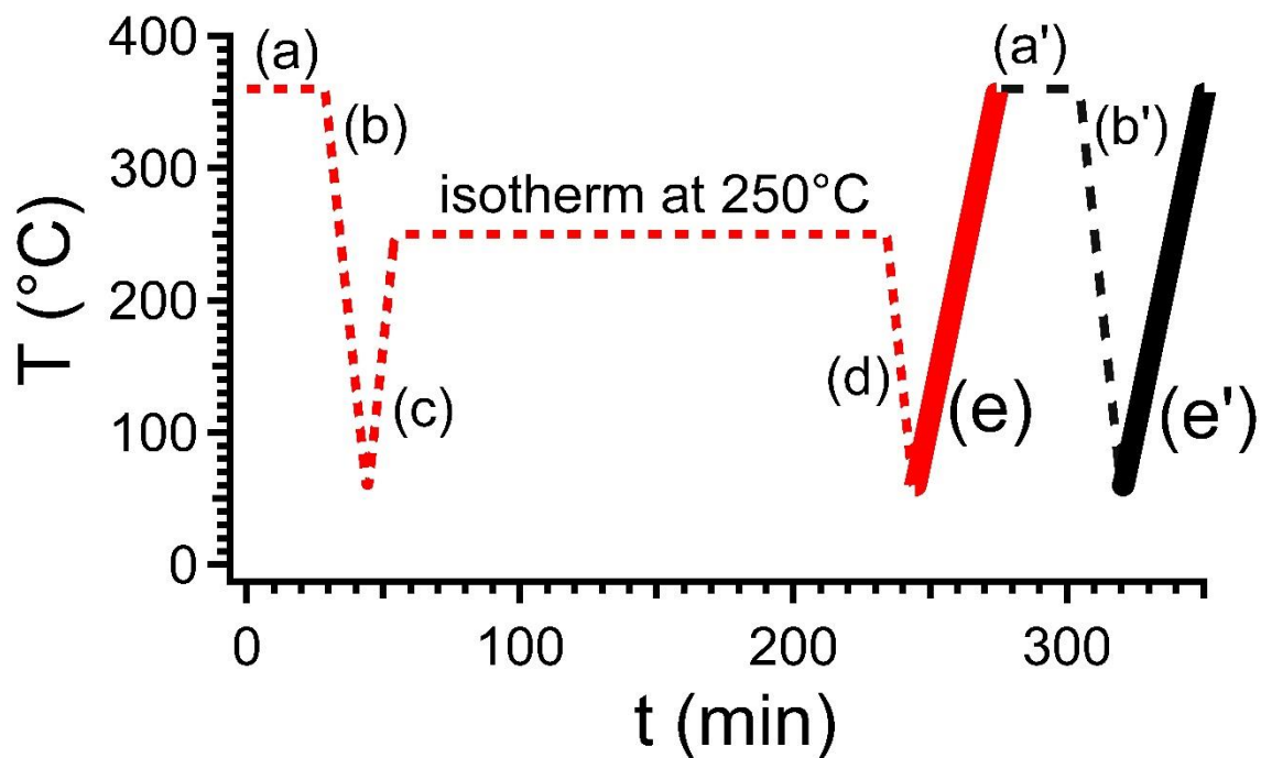
Figure 3: Thermal history applied to crystallized samples (in red) and amorphous samples (in black).
