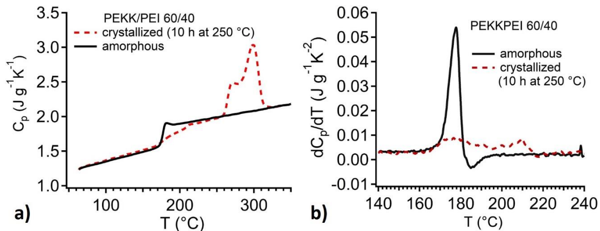
Figure 6. a) Variation in the heat capacity (in \text{J g}^{-1}\text{K}^{-1} ) of the PEKK/PEI blend that contains 60 wt % PEKK with temperature measured by applying a heating rate of 10^\circ\text{C}/\text{min} . b) Corresponding variation in the derivative of the heat capacity dC_p/dT with respect to temperature with temperature. The black line corresponds to the signals measured on the fully amorphous blend, while the red dotted line shows the signals measured on the blend maximally crystallized (i.e., for 10 h) at 250^\circ\text{C} .
