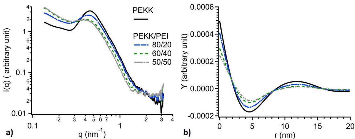
Figure 9. a) Variation in the intensity scattered by PEKK/PEI blends maximally crystallized at 250°C with the scattering vector q . b) Corresponding correlation function as a function of the distance r .
