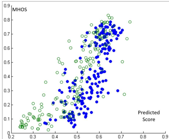
Figure 4: Scatter plot of the predicted quality scores employing our proposed method against subjective MHOS scores on the ITESOPT dataset. Blue and Green indicate JPEG and JPEG2000 distortions respectively.
