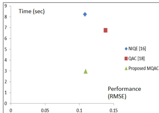
Figure 6: Trade-off between time and accuracy concerning RMSE of the considered NR DIQA methods on the ITESOFT dataset.
