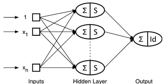
Fig. 4. Neural network with one hidden layer.
