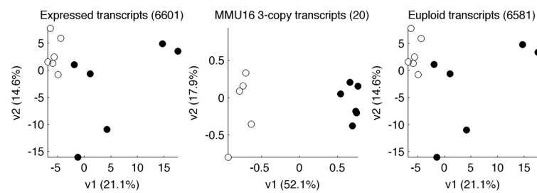
Figure 1.10 PCA of the data described in Saran et al. (Saran et al. , 2003).
